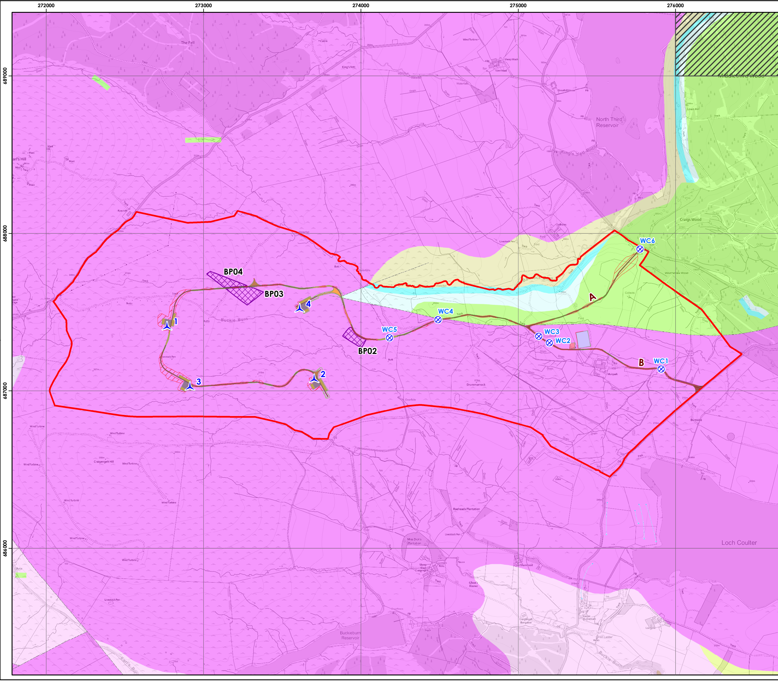
Figure 8-2b Bedrock Geology
