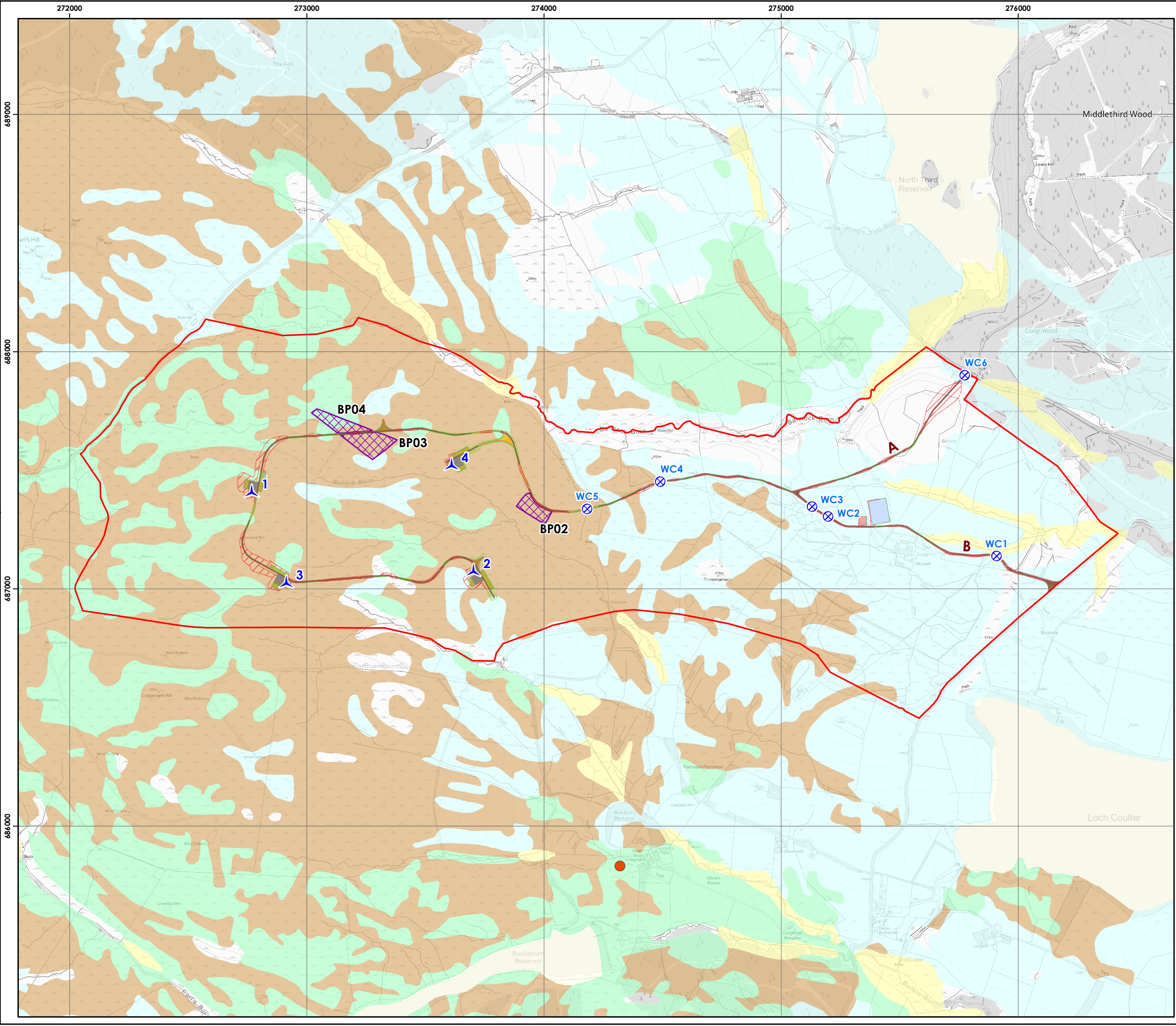
Figure 8-2a Superficial Geology
